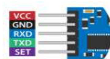
Figura 4.33 Pinout módulo HC-12
